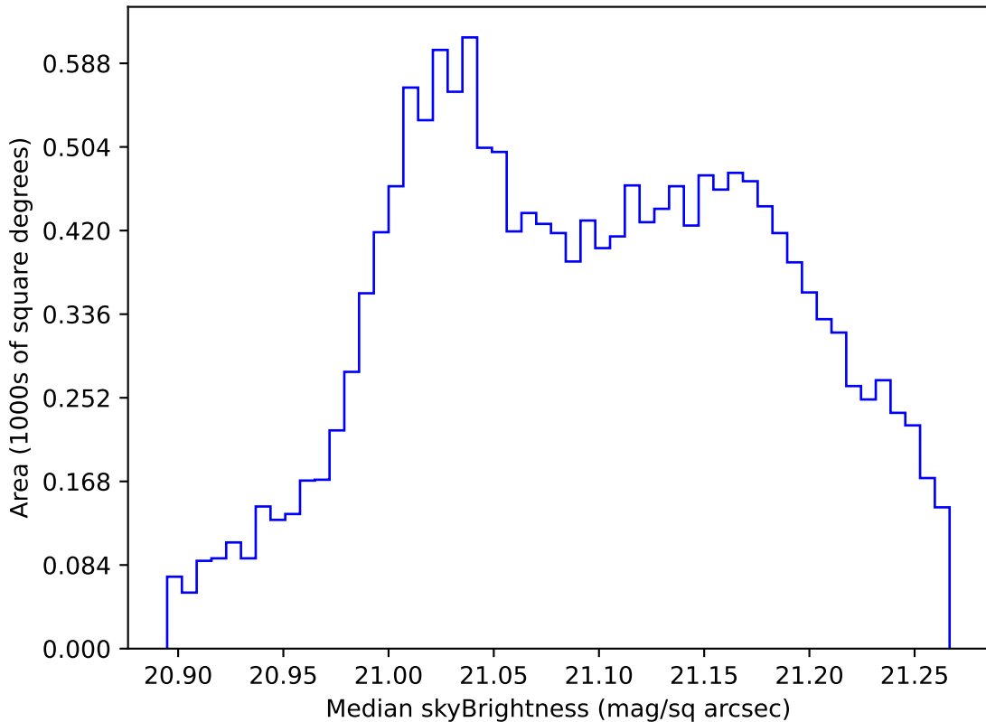
internal_u_expt38_nscale0.9v3.4_10yrs WFD r band: Median skyBrightness
