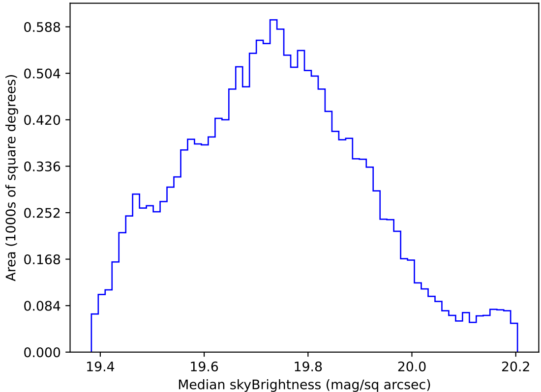
internal_u_expt38_nscale0.9v3.4_10yrs WFD all bands: Median skyBrightness
