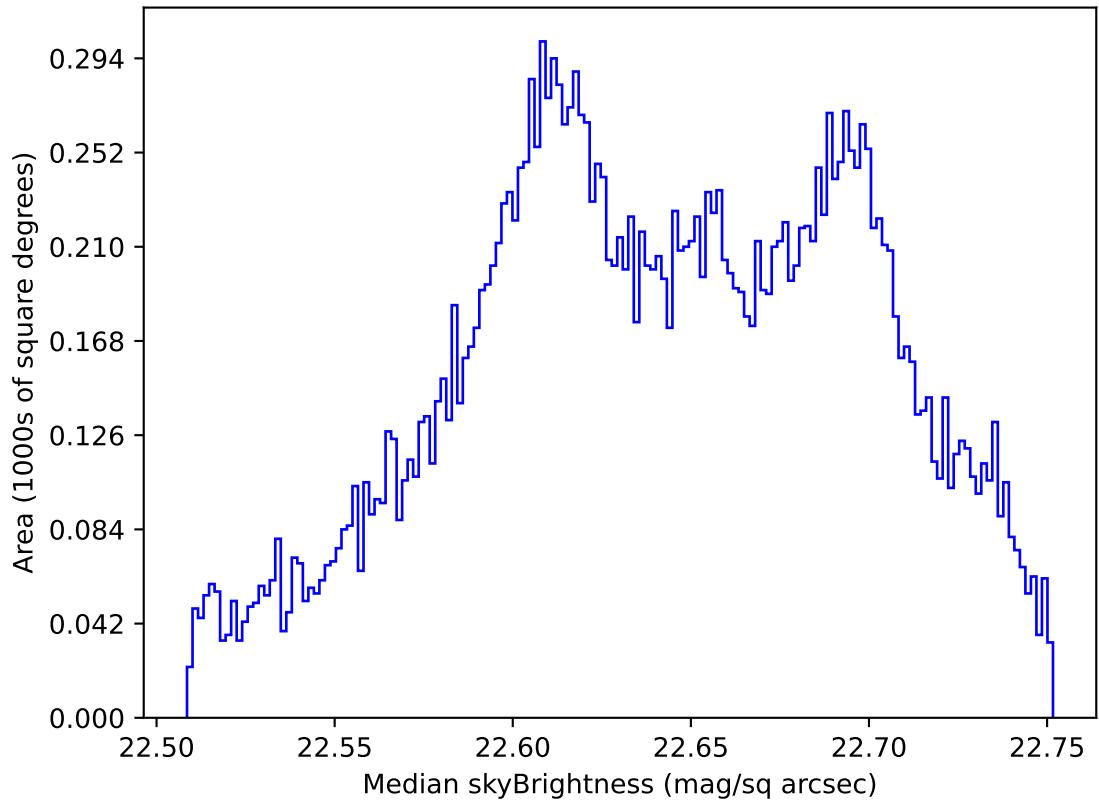
internal_u_expt38_nscale0.9v3.4_10yrs All sky u band: Median skyBrightness
