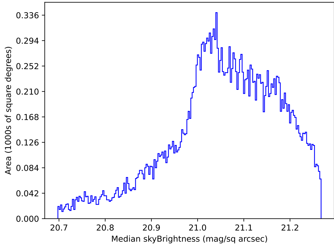
internal_u_expt38_nscale0.9v3.4_10yrs All sky r band: Median skyBrightness
