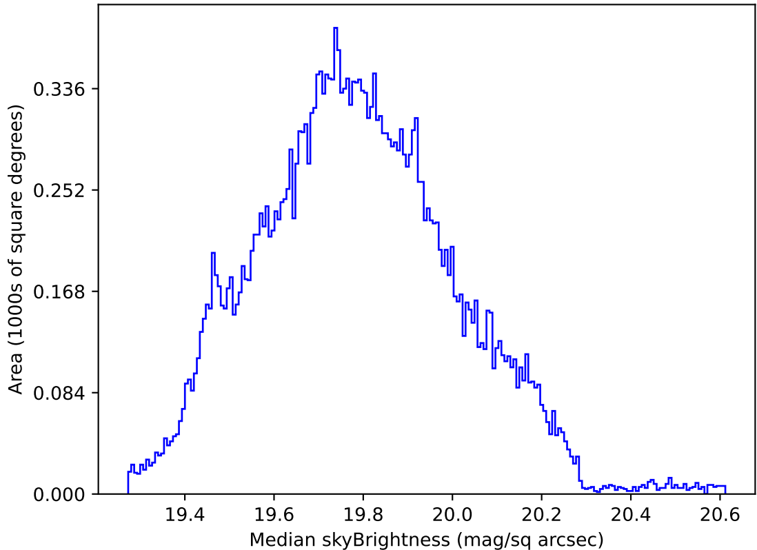
internal_u_expt38_nscale0.9v3.4_10yrs All sky all bands: Median skyBrightness
