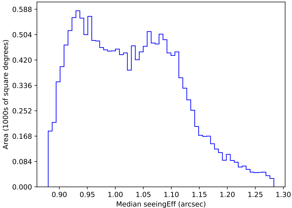
internal_u_expt38_nscale0.9v3.4_10yrs WFD r band: Median seeingEff
