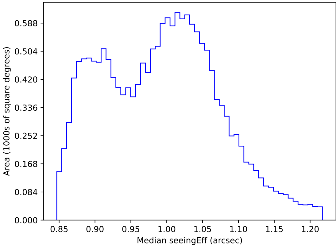
internal_u_expt38_nscale0.9v3.4_10yrs WFD i band: Median seeingEff
