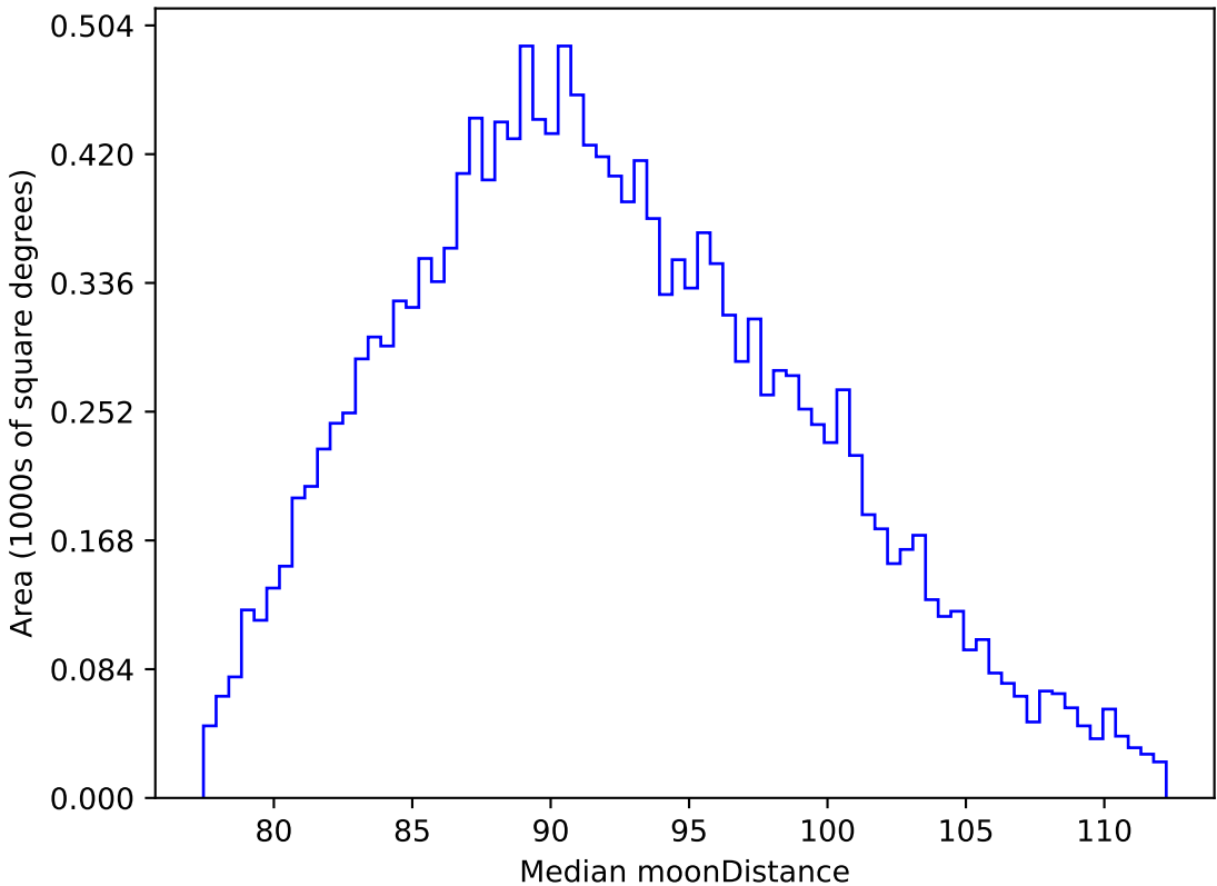
internal_u_expt38_nscale0.9v3.4_10yrs WFD i band: Median moonDistance
