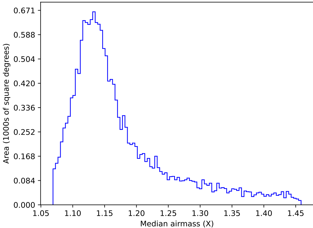
internal_u_expt38_nscale0.9v3.4_10yrs WFD u band: Median airmass
