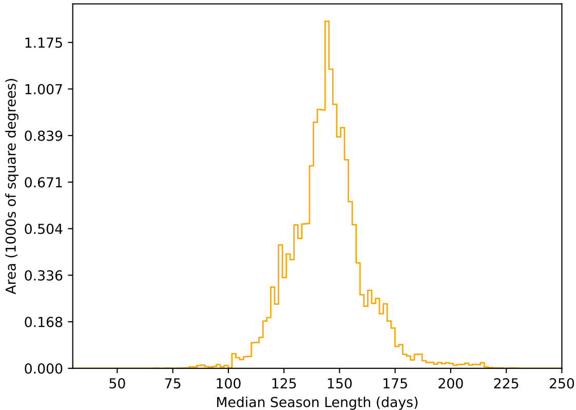
internal_u_expt38_nscale0.9v3.4_10yrs WFD r band: Median Season Length
