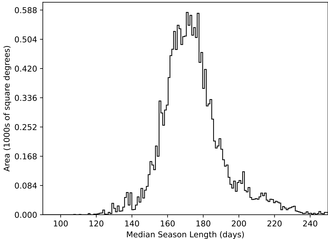
internal_u_expt38_nscale0.9v3.4_10yrs WFD all bands: Median Season Length
