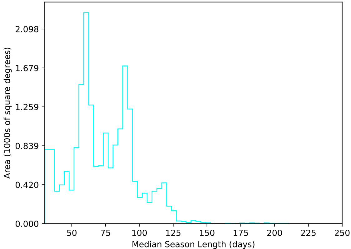
internal_u_expt38_nscale0.9v3.4_10yrs All sky u band: Median Season Length
