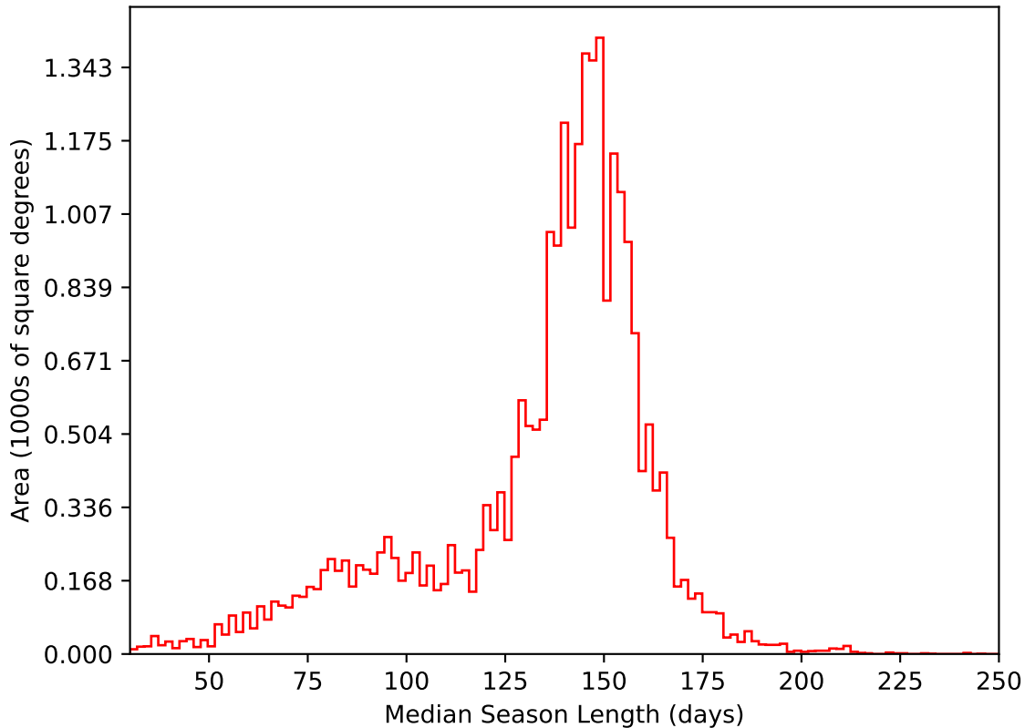
internal_u_expt38_nscale0.9v3.4_10yrs All sky i band: Median Season Length
