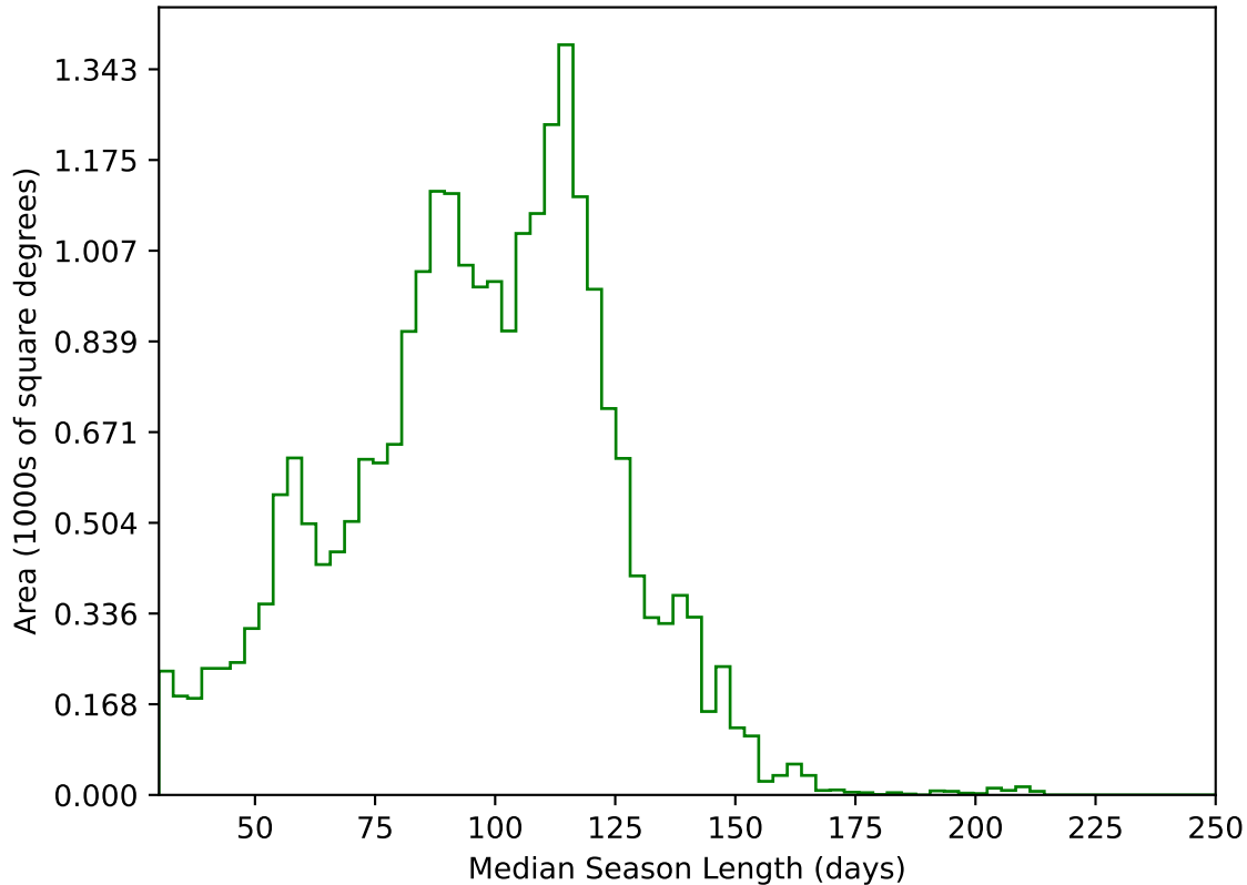
internal_u_expt38_nscale0.9v3.4_10yrs All sky g band: Median Season Length
