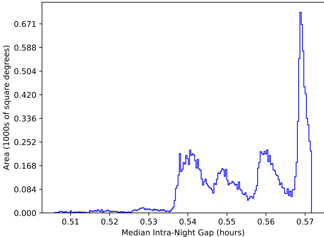
internal_u_expt38_nscale0.9v3.4_10yrs WFD: Median Intra-Night Gap
