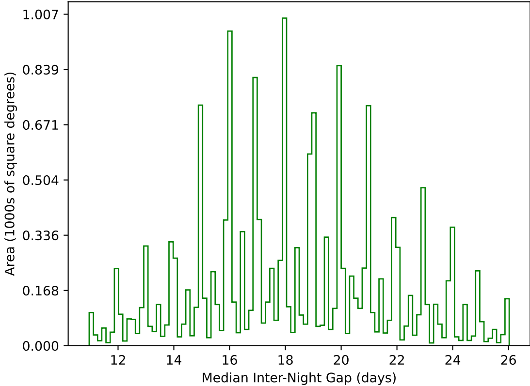
internal_u_expt38_nscale0.9v3.4_10yrs WFD g band: Median Inter-Night Gap
