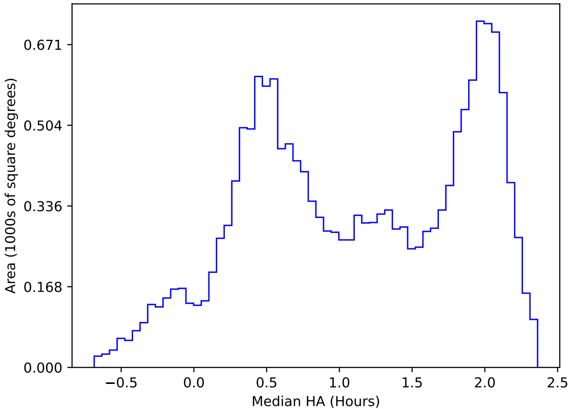
internal_u_expt38_nscale0.9v3.4_10yrs WFD z band: Median HA
