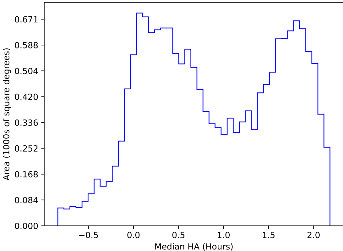
internal_u_expt38_nscale0.9v3.4_10yrs WFD r band: Median HA
