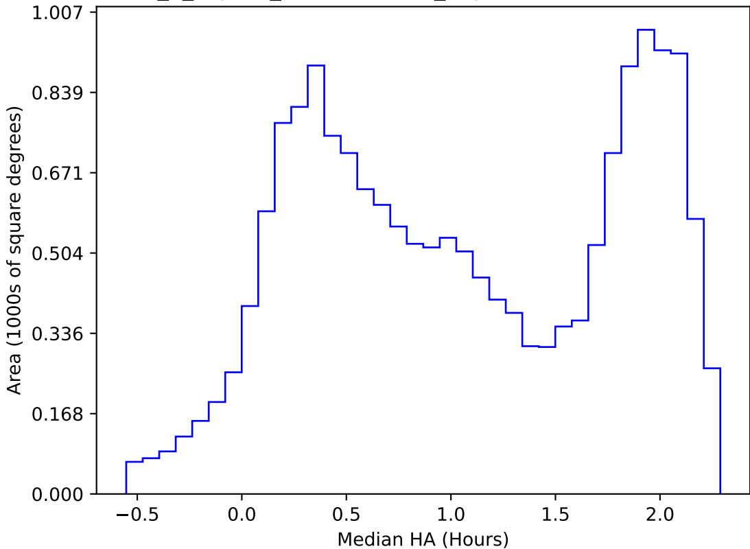
internal_u_expt38_nscale0.9v3.4_10yrs WFD i band: Median HA
