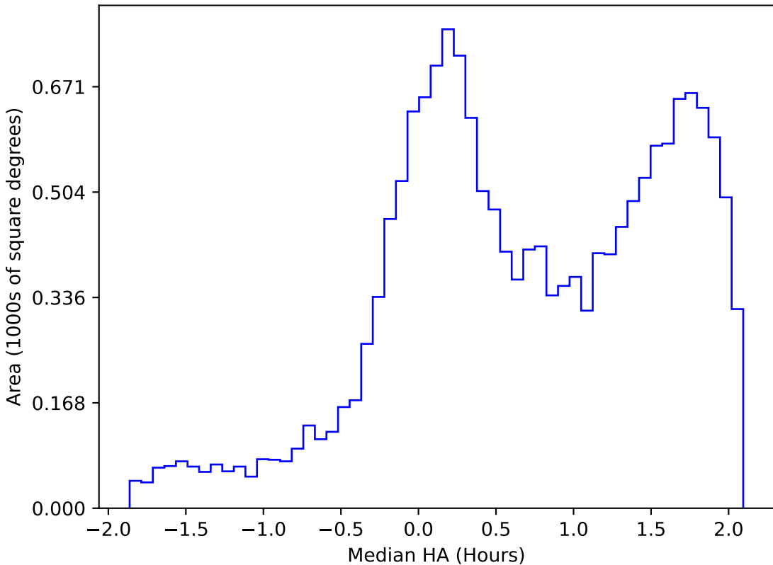
internal_u_expt38_nscale0.9v3.4_10yrs WFD g band: Median HA
