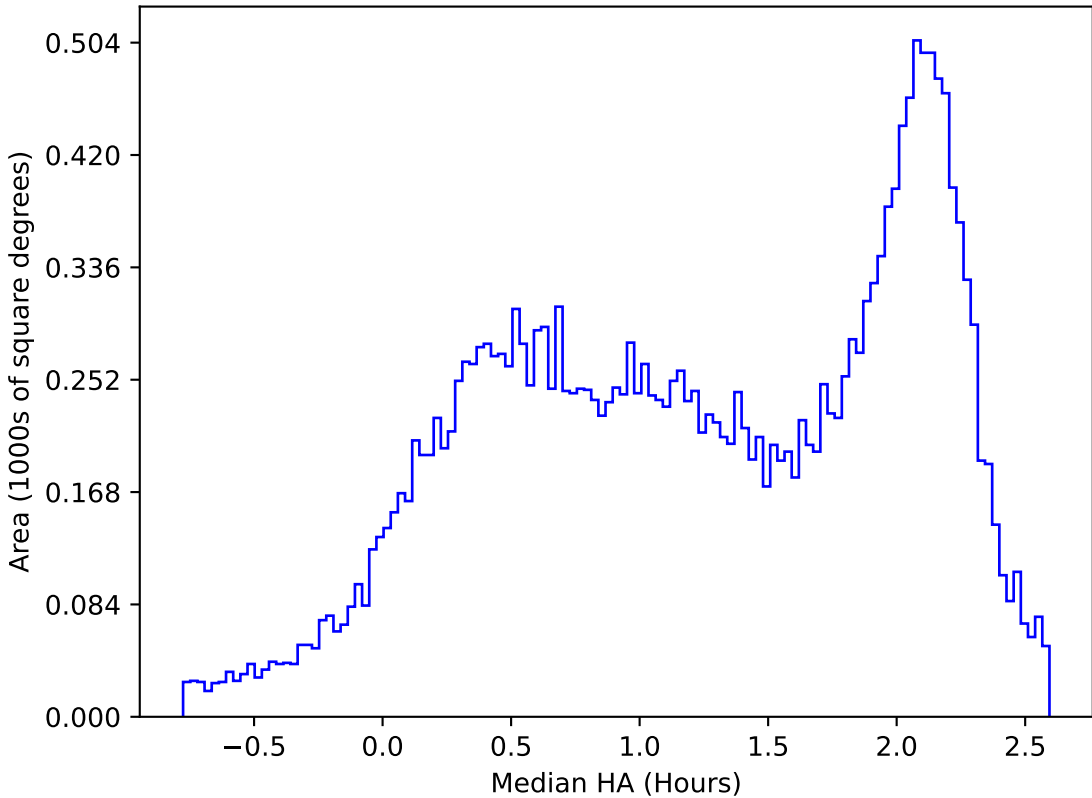
internal_u_expt38_nscale0.9v3.4_10yrs All sky y band: Median HA
