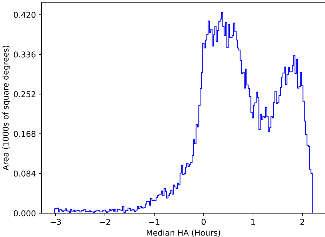
internal_u_expt38_nscale0.9v3.4_10yrs All sky r band: Median HA
