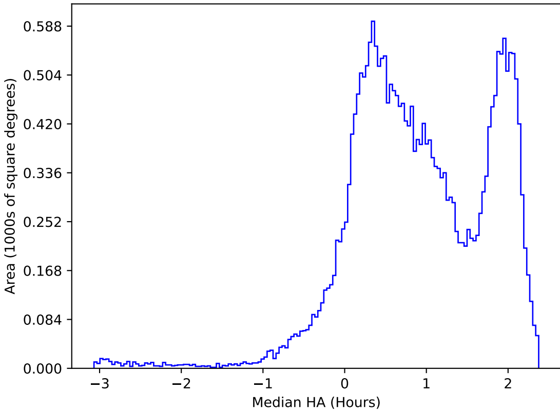
internal_u_expt38_nscale0.9v3.4_10yrs All sky i band: Median HA
