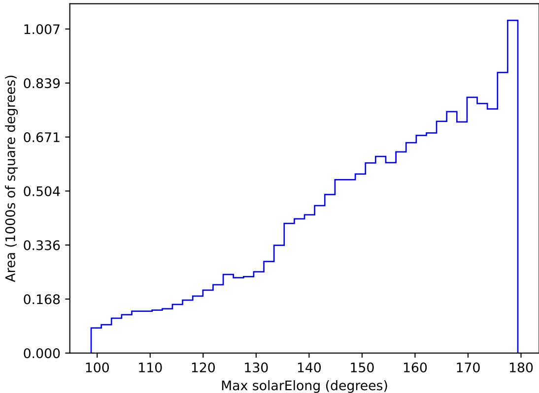
internal_u_expt38_nscale0.9v3.4_10yrs WFD r band: Max solarElong
