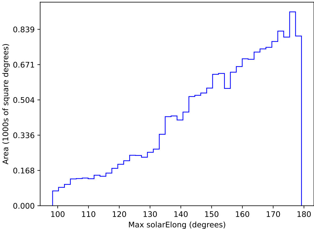
internal_u_expt38_nscale0.9v3.4_10yrs WFD g band: Max solarElong
