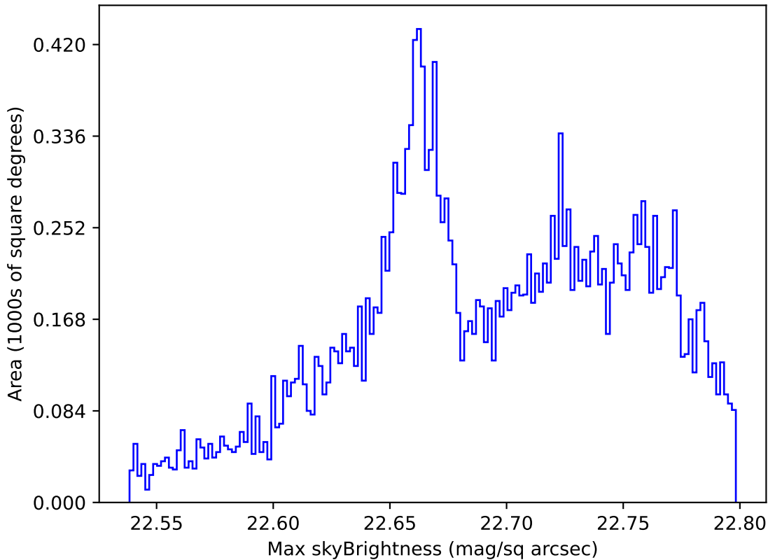
internal_u_expt38_nscale0.9v3.4_10yrs All sky u band: Max skyBrightness
