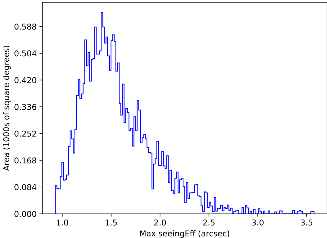
internal_u_expt38_nscale0.9v3.4_10yrs Yr 1 u band: Max seeingEff
