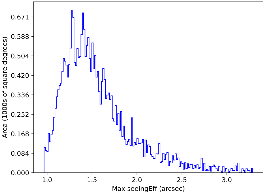
internal_u_expt38_nscale0.9v3.4_10yrs Yr 1 i band: Max seeingEff
