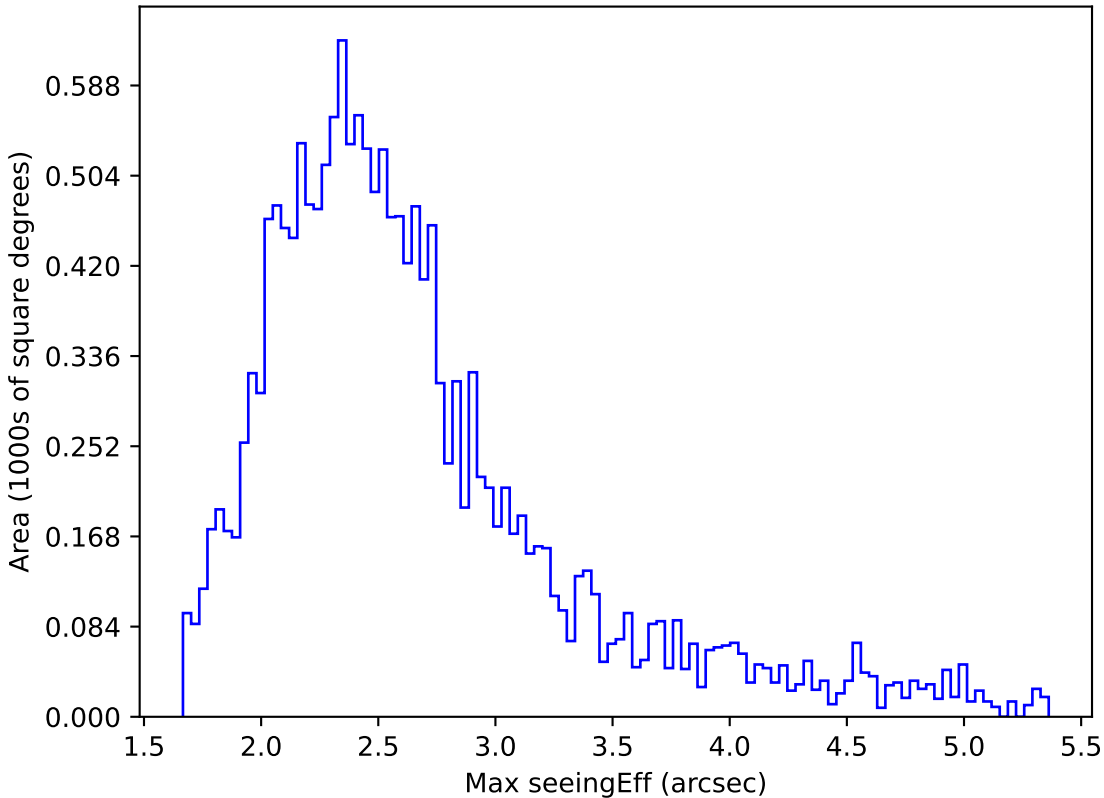
internal_u_expt38_nscale0.9v3.4_10yrs WFD z band: Max seeingEff
