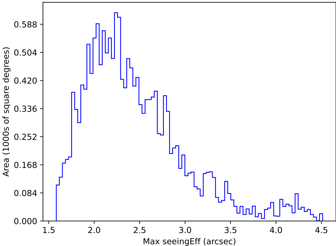
internal_u_expt38_nscale0.9v3.4_10yrs WFD y band: Max seeingEff
