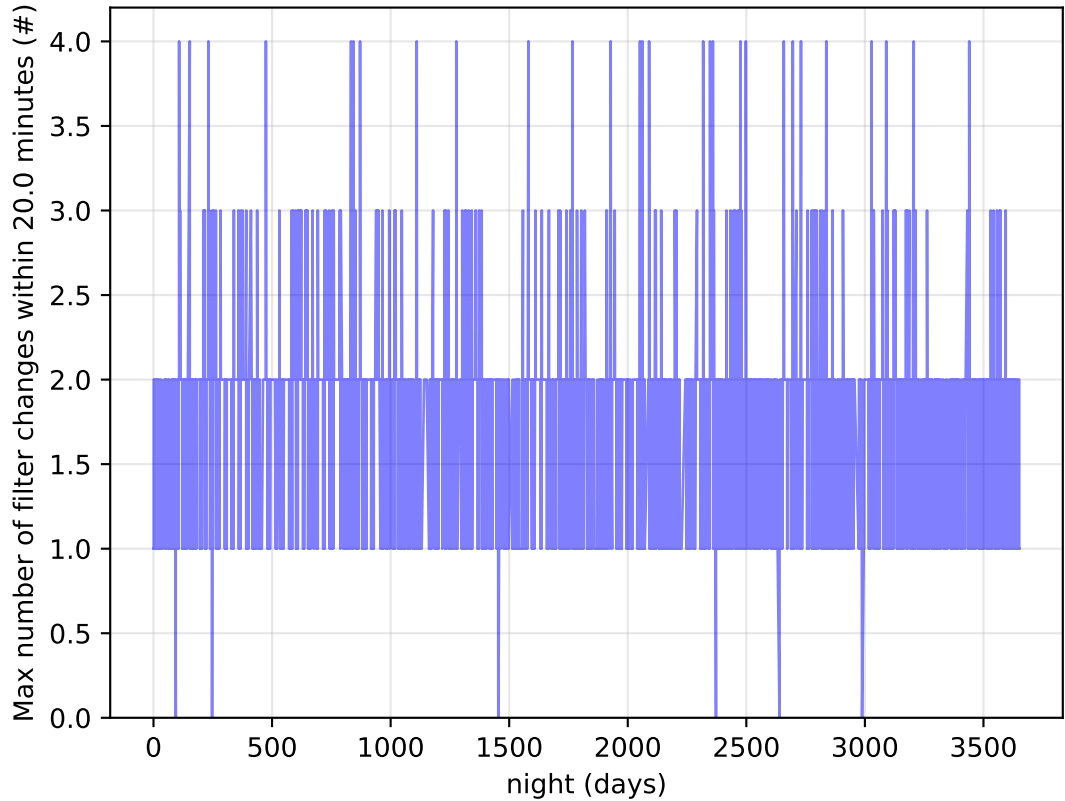
internal_u_expt38_nscale0.9v3.4_10yrs Per Night: Max number of filter changes within 20.0 minutes
