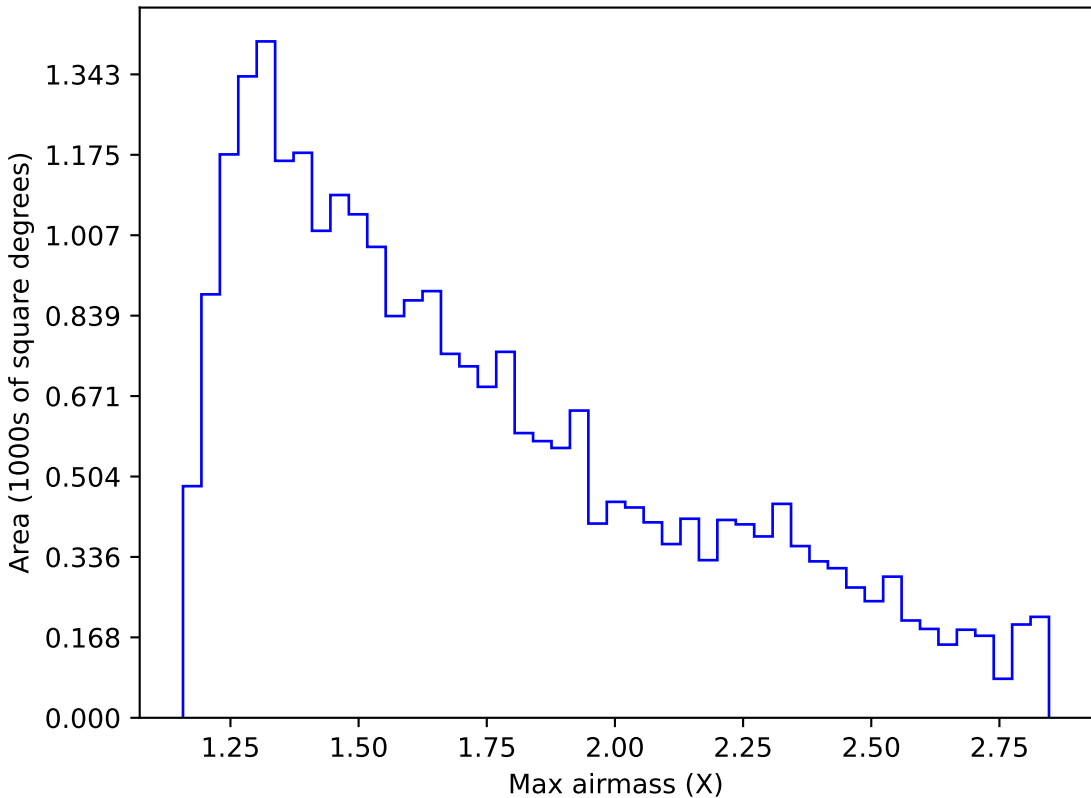
internal_u_expt38_nscale0.9v3.4_10yrs Yr 1 z band: Max airmass
