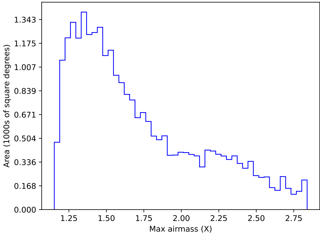
internal_u_expt38_nscale0.9v3.4_10yrs Yr 1 i band: Max airmass
