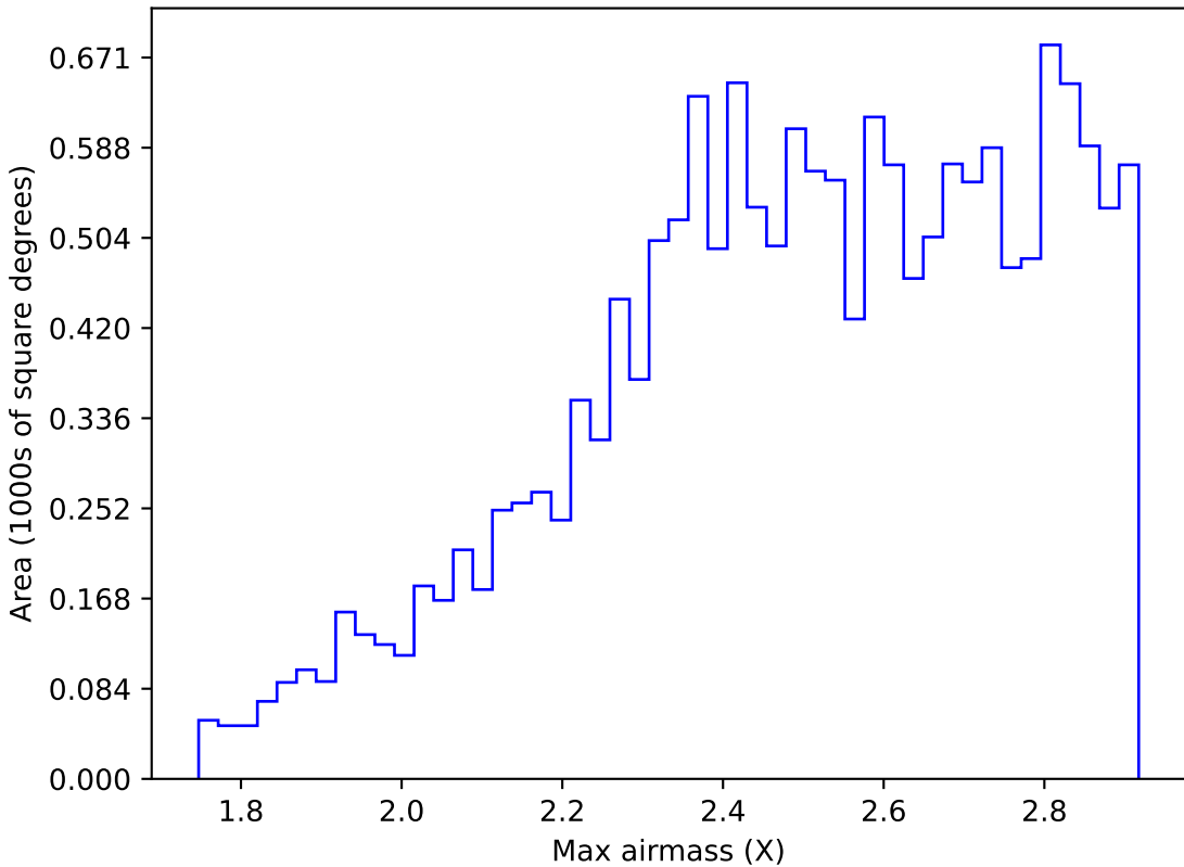
internal_u_expt38_nscale0.9v3.4_10yrs WFD z band: Max airmass
