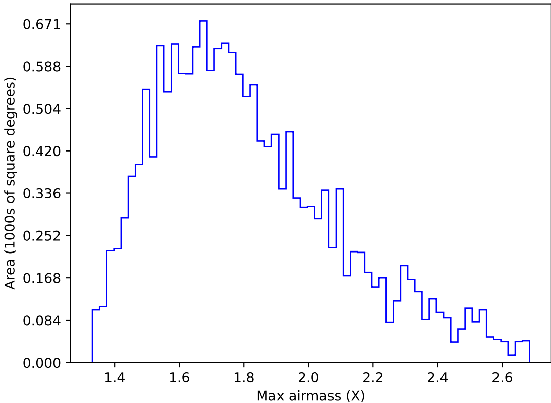
internal_u_expt38_nscale0.9v3.4_10yrs WFD u band: Max airmass
