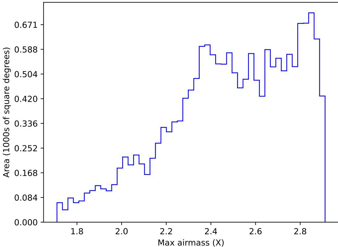
internal_u_expt38_nscale0.9v3.4_10yrs WFD i band: Max airmass
