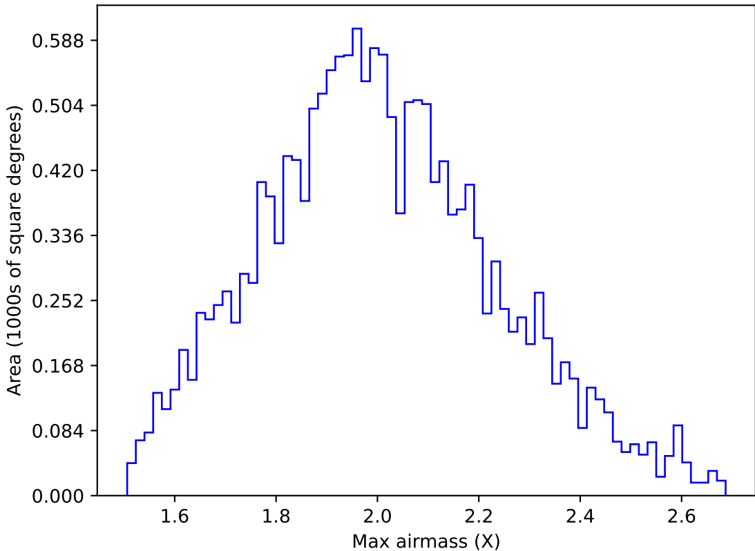
internal_u_expt38_nscale0.9v3.4_10yrs WFD g band: Max airmass
