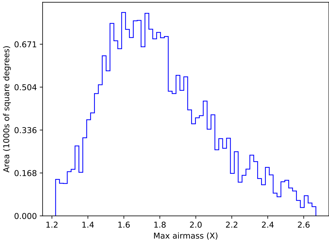
internal_u_expt38_nscale0.9v3.4_10yrs All sky u band: Max airmass
