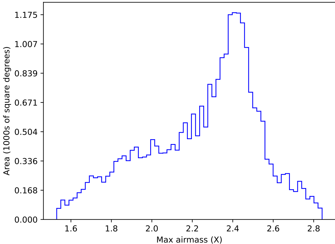
internal_u_expt38_nscale0.9v3.4_10yrs All sky r band: Max airmass
