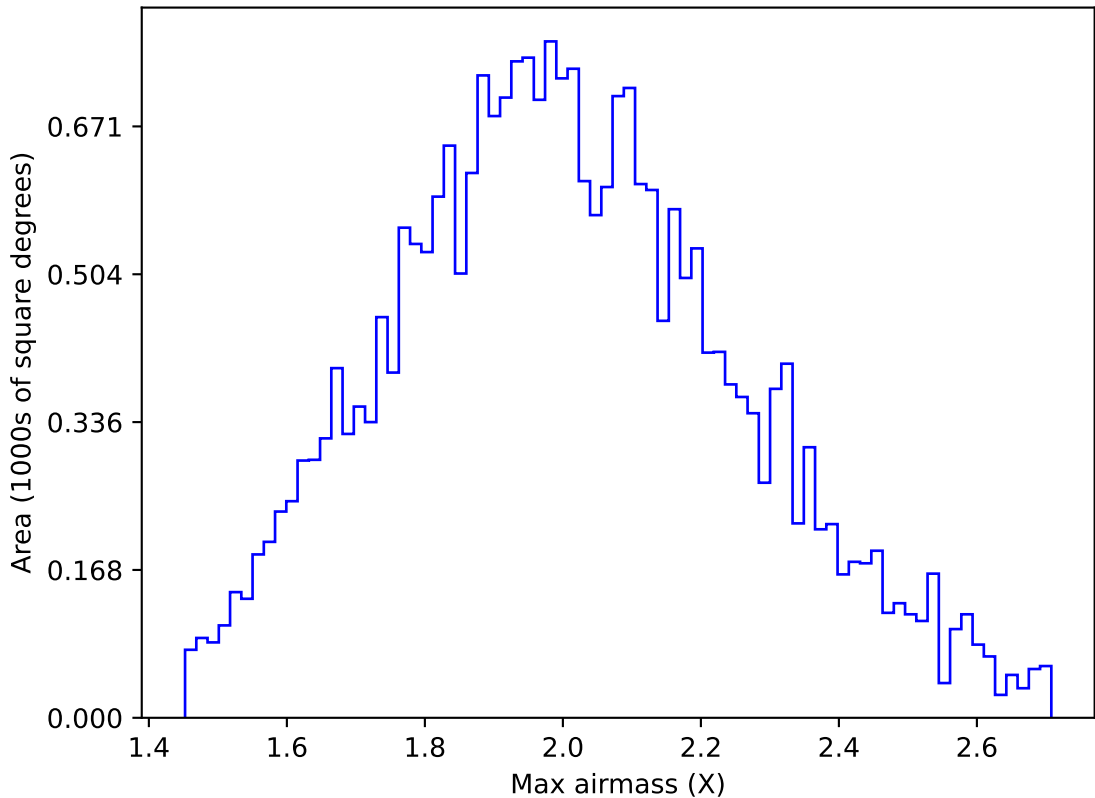
internal_u_expt38_nscale0.9v3.4_10yrs All sky g band: Max airmass
