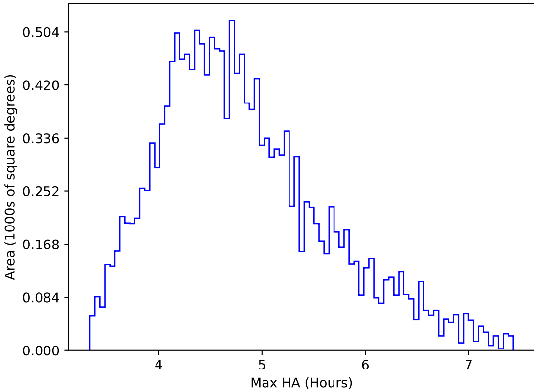
internal_u_expt38_nscale0.9v3.4_10yrs WFD y band: Max HA
