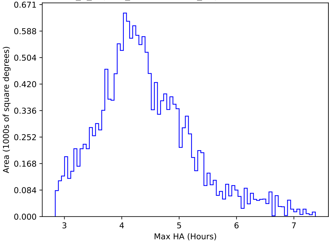
internal_u_expt38_nscale0.9v3.4_10yrs WFD r band: Max HA
