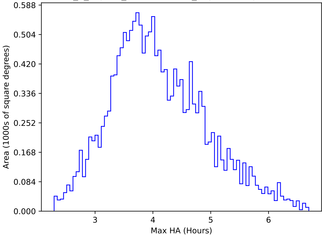
internal_u_expt38_nscale0.9v3.4_10yrs WFD g band: Max HA
