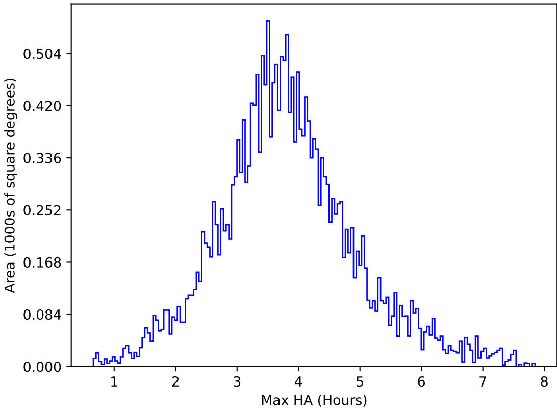
internal_u_expt38_nscale0.9v3.4_10yrs All sky u band: Max HA
