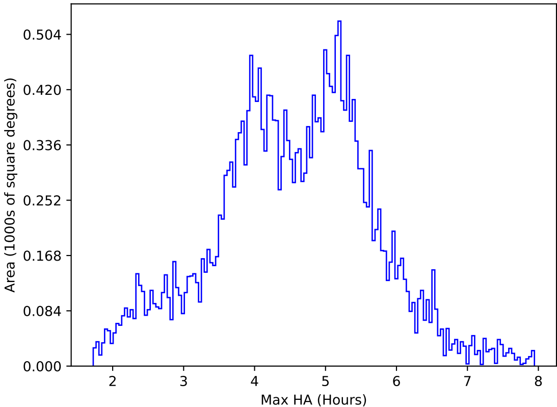
internal_u_expt38_nscale0.9v3.4_10yrs All sky i band: Max HA
