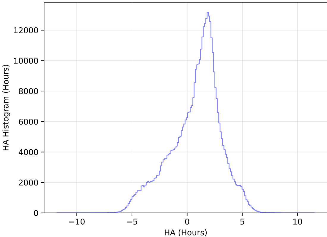
internal_u_expt38_nscale0.9v3.4_10yrs WFD z band: HA Histogram
