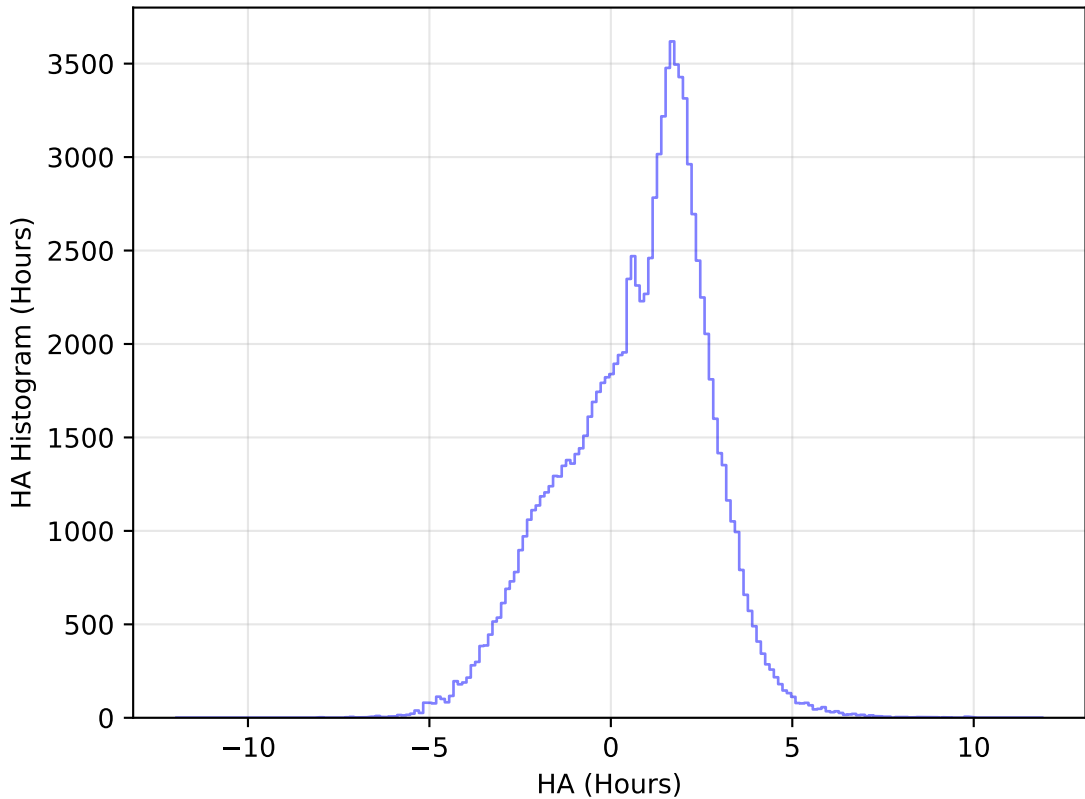
internal_u_expt38_nscale0.9v3.4_10yrs WFD u band: HA Histogram
