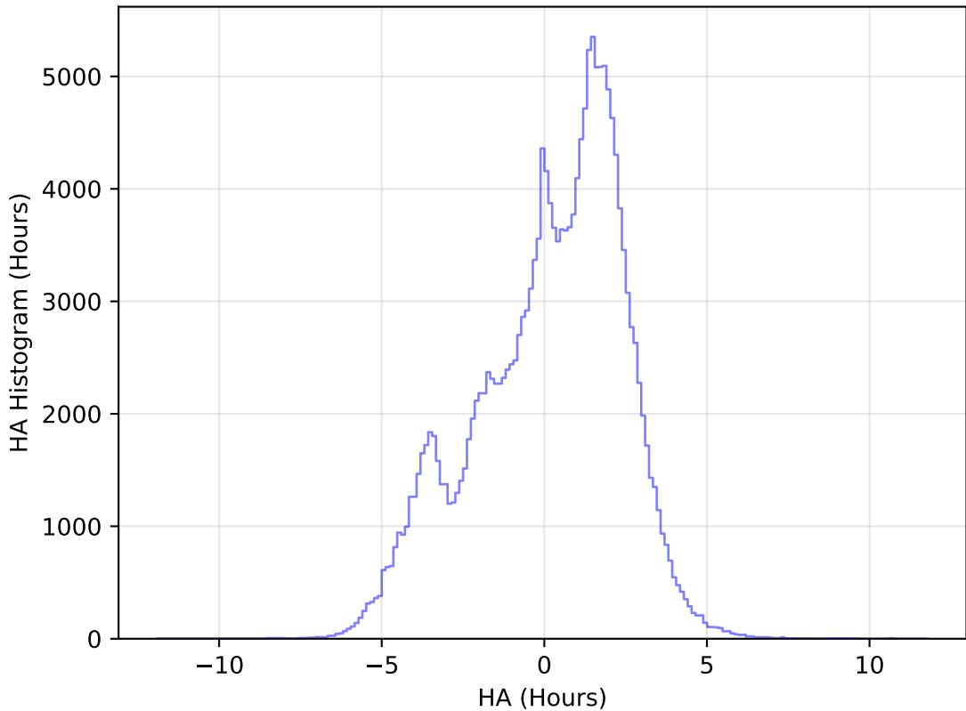
internal_u_expt38_nscale0.9v3.4_10yrs WFD g band: HA Histogram
