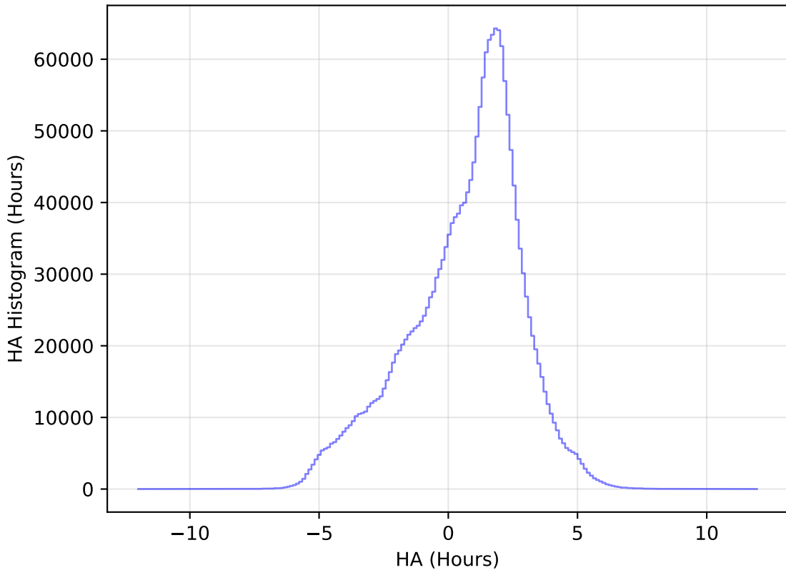
internal_u_expt38_nscale0.9v3.4_10yrs WFD all bands: HA Histogram
