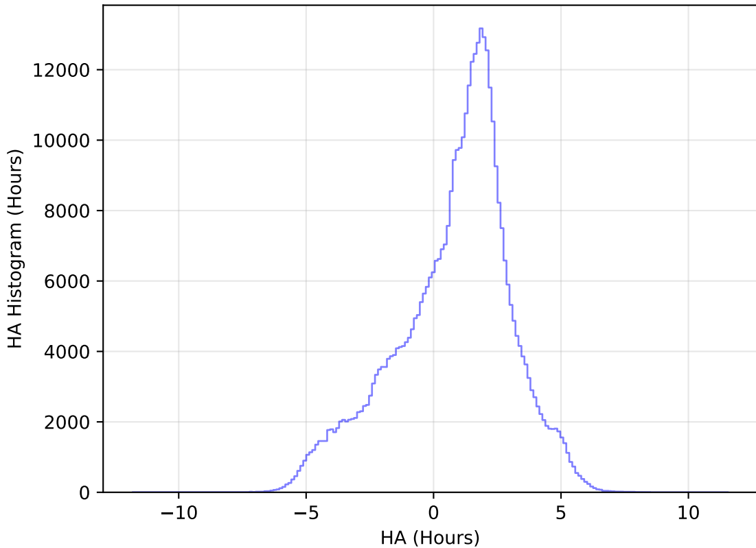
internal_u_expt38_nscale0.9v3.4_10yrs All sky z band: HA Histogram
